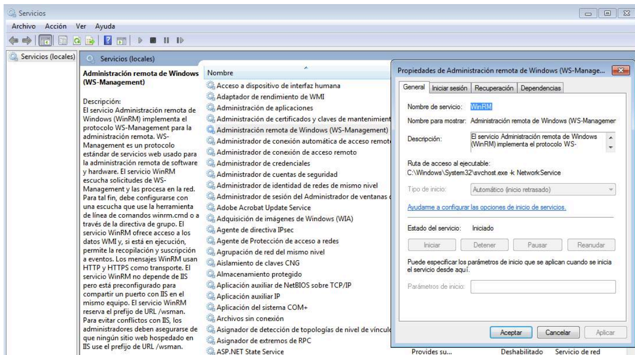
Figura 7: Servicio WinRM
